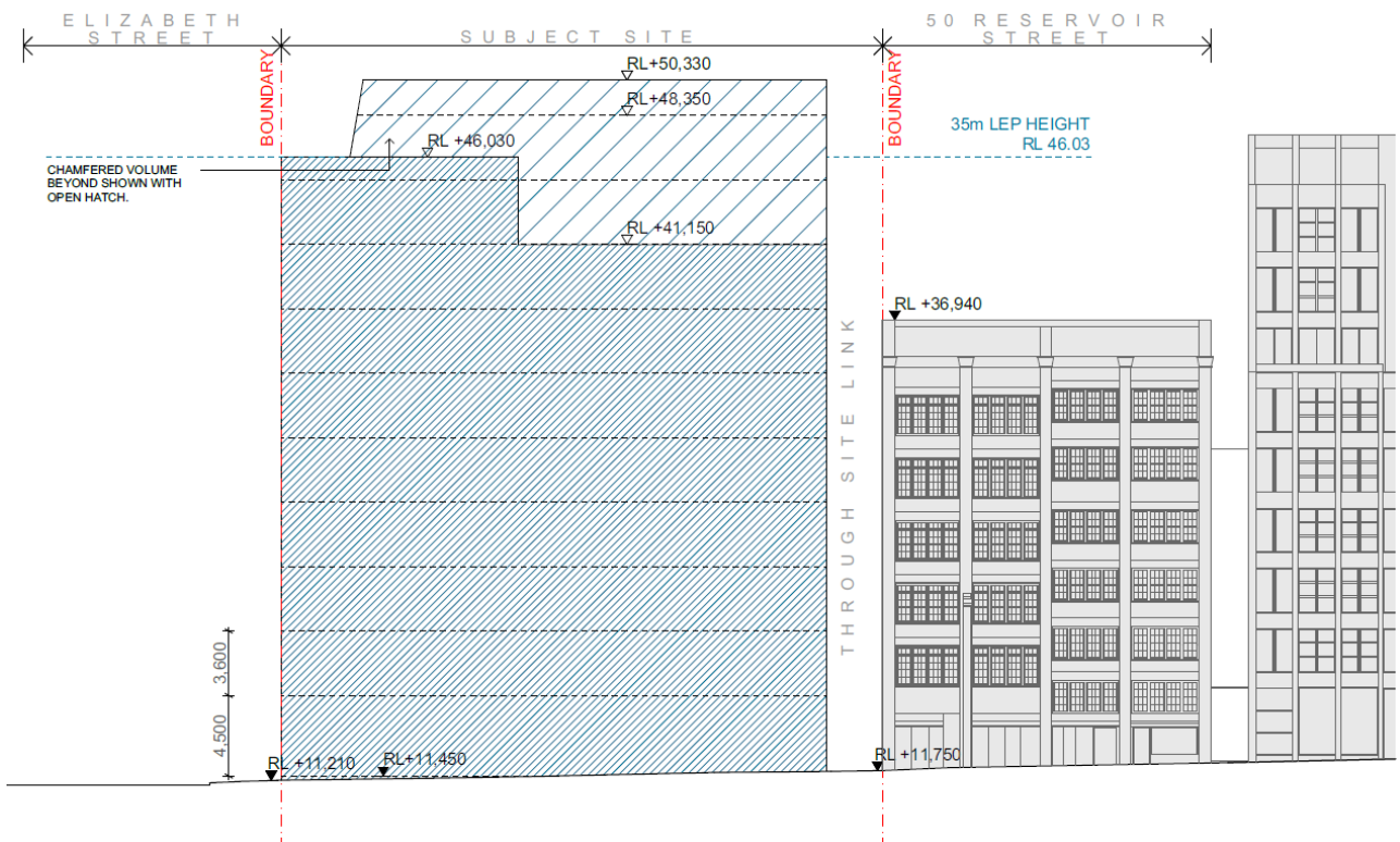
Figure 6.X 232-240 Elizabeth Street, Surry Hills - Maximum building envelope axonometric
