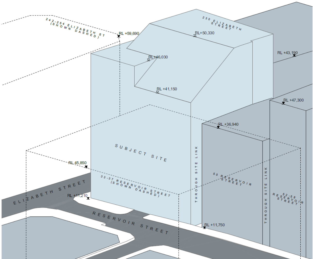
Figure 6.X 232-240 Elizabeth Street, Surry Hills - Maximum building envelope southern elevation
